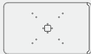
VESA mount 75x75 and 100x100
